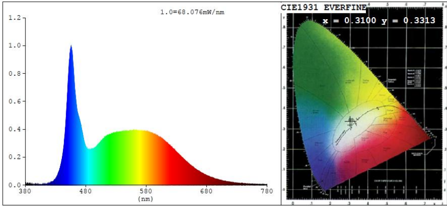
CCT 6500 K
